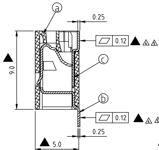
Section P-P
