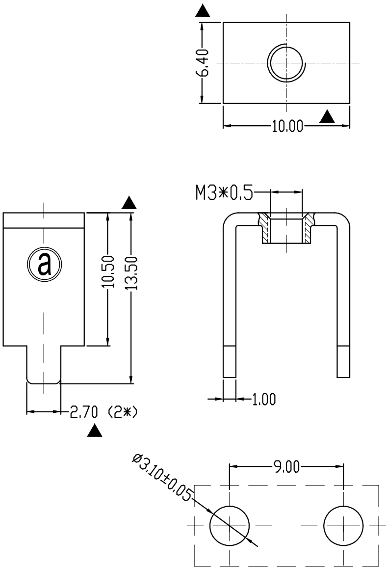
PCB LAYOUT
