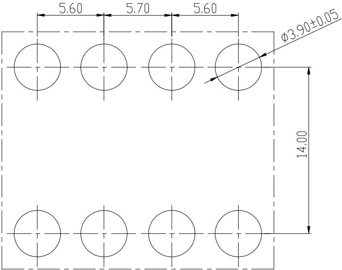
PCB LAYOUT
