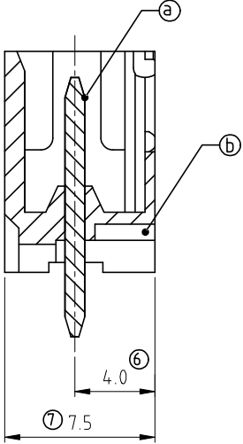
SECTION P-P
