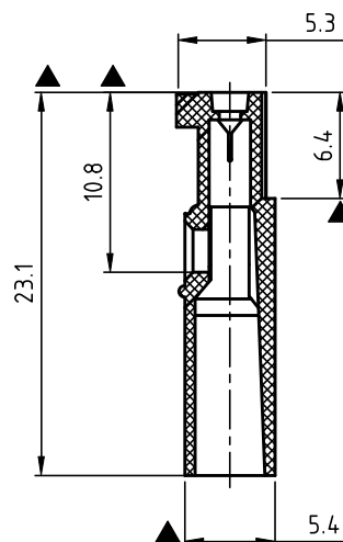
Section P-P
