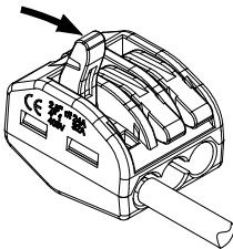
Step 3. 按下压板锁线 Push the Lever to lock
