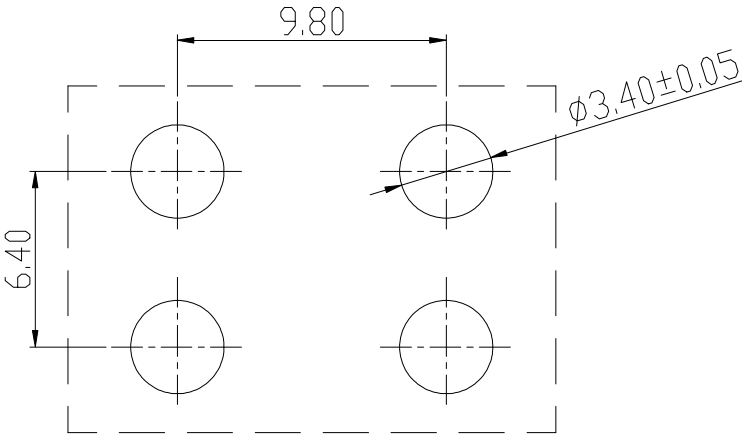
PCB LAYOUT
